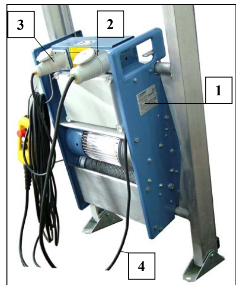
Fig. 6 Winde LIFT 250 COMFORT
