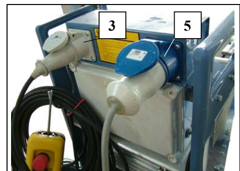
Fig. 7 Winde FIXLIFT 250
