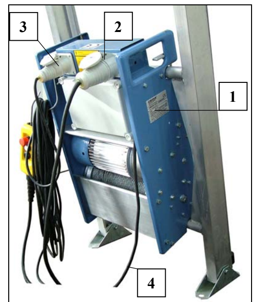
Fig. 6 Winde LIFT 250 COMFORT
